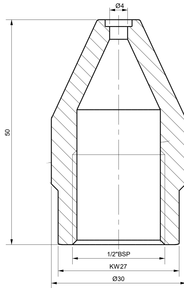
Section B-B
