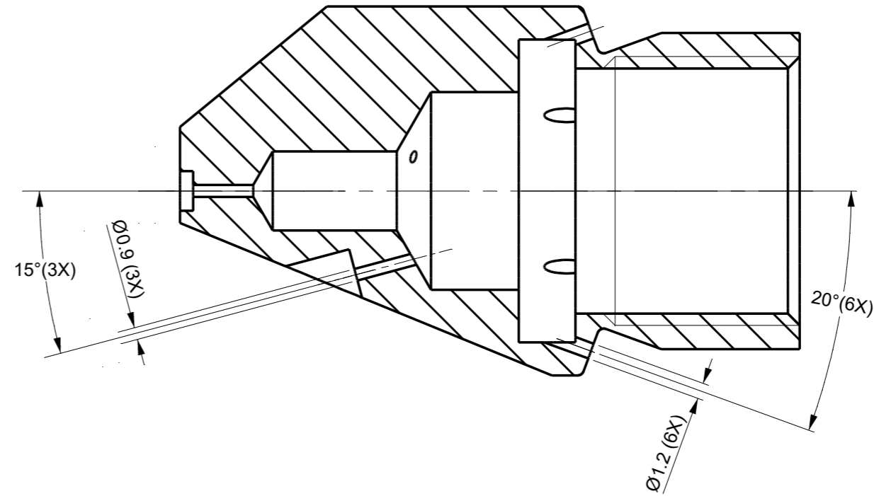
Section C-C
