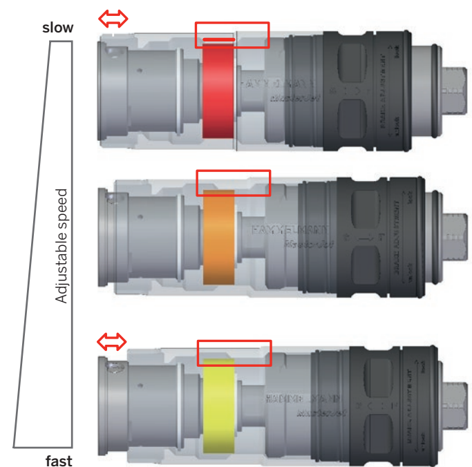
Brake adjustment by simple adjustment of the protective sleeve
